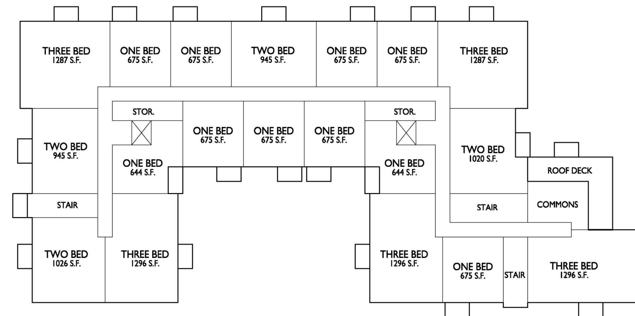
FIFTH FLOOR
