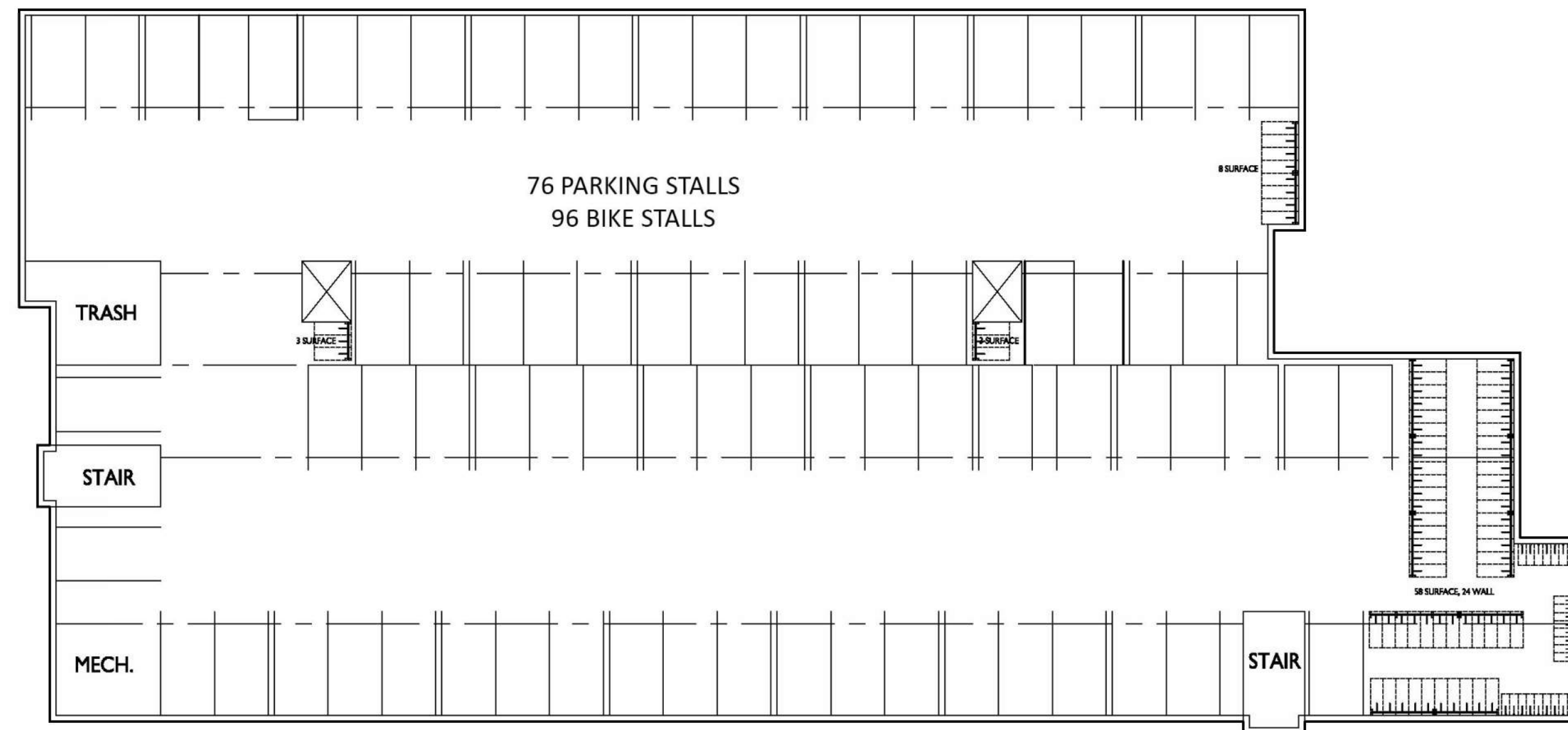
BASEMENT
