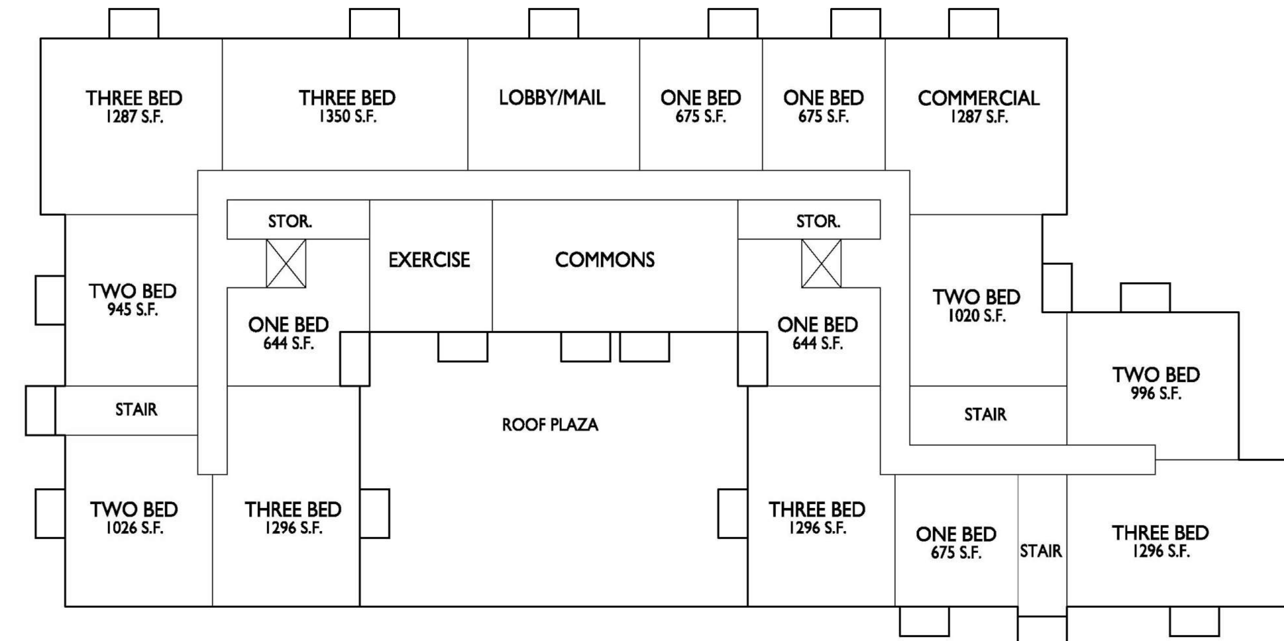
FIRST FLOOR
